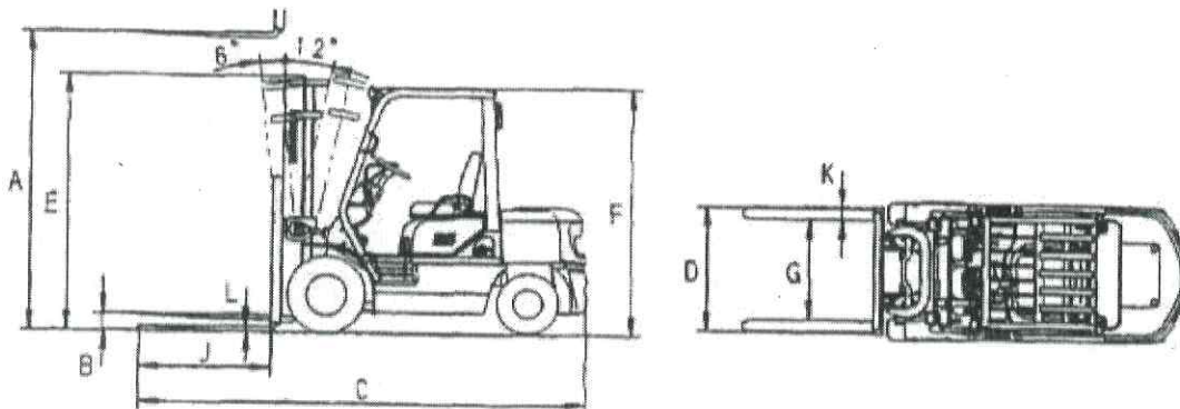
Dimension chart
