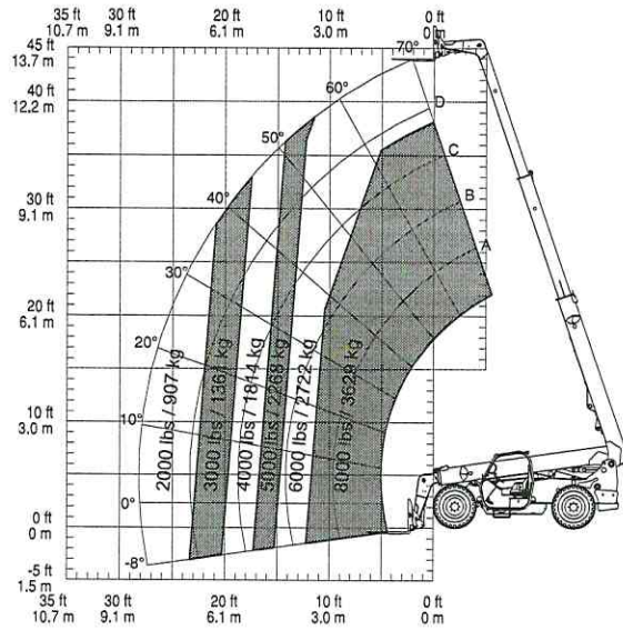
GTH-844 Standard Carriage
