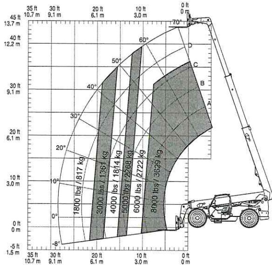
GTH-844 Rotate Carriage
