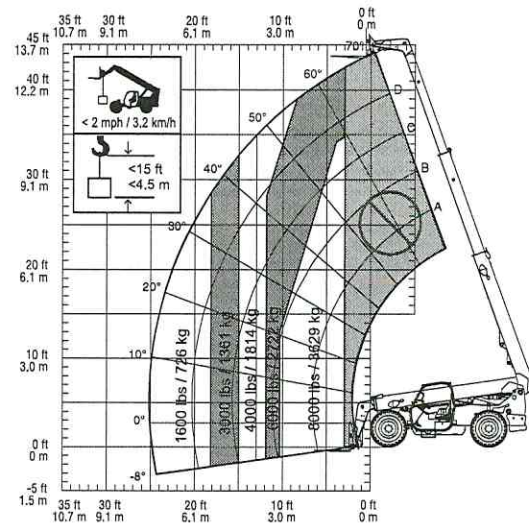
GTH-844 Swing Carriage
